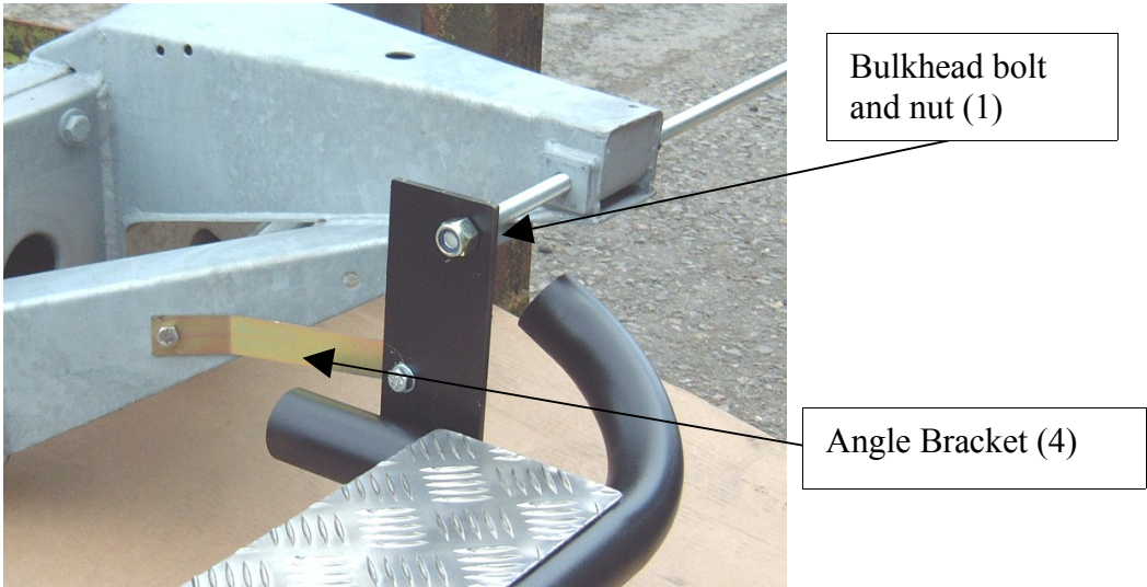
Rear Mounting showing outrigger
